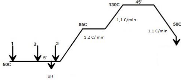
Figure 4. Dyeing diagram
