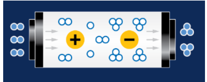
Figure 2. Ozone formation by Corona Discharge method [10]
