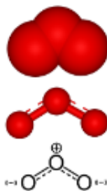
Figure 1. Ozone molecule structure[10]
